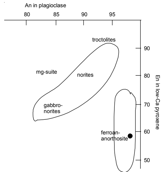
Figure 4: Plagioclase-low-Ca pyroxene diagram showing that 15415 plots in field of ferroan anorthosite.
