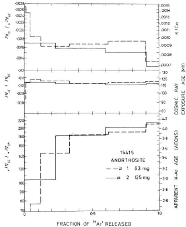
Figure 7: Argon plateau age for 15415 as determined by Turner et al. 1972.
