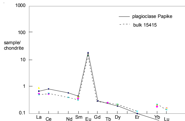
Figure 5: Normalized rare-earth-element composition diagram for 15415 plagioclase and whole rock.
