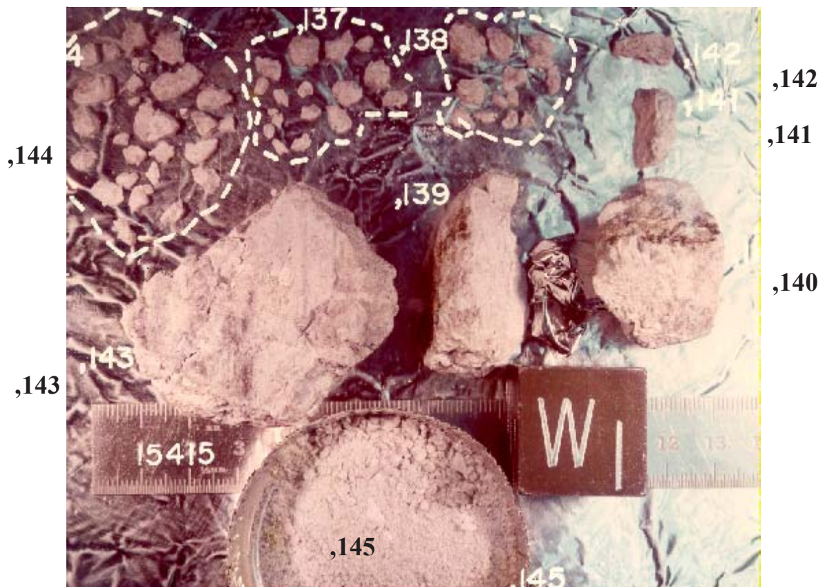
Figure 9: Subdivision of 15415,0 yielding ,143, ,139 ,140 and pieces and crumbs. NASA photo # S75-32659. Cube is 1 inch.
