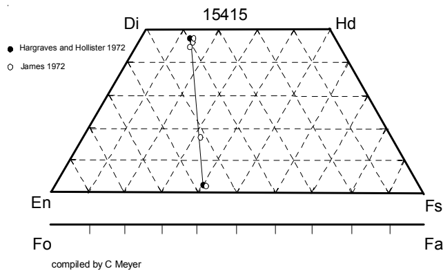
Figure 3: Pyroxene composition for 15415 (data from James 1972, Hargraves and Hollister 1972).
