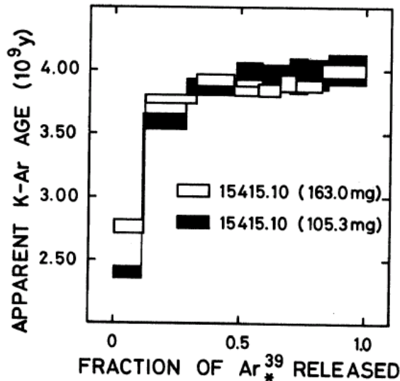
Figure 6: Argon plateau age for 15415 (from Stettler et al. 1973).
